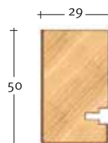
Art. 3022 Profilo Architrave Architrave profile
