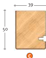
Art. 3023 Profilo Architrave Architrave profile
