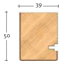
Art. 3023 Profilo Architrave Architrave profile
