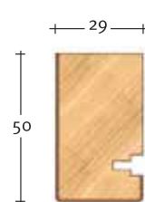
Art. 3022 Profilo Architrave Architrave profile
