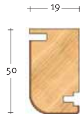
Art. 3082 Profilo Architrave Architrave profile
