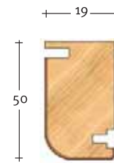
Art. 3082 Profilo Architrave Architrave profile
