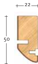
Art. 3027 Profilo Architrave Architrave profile
